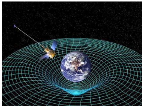
Artist concept of Gravity Probe B orbiting the Earth to measure space-time, a four-dimensional description of the universe including height, width, length, and time.
